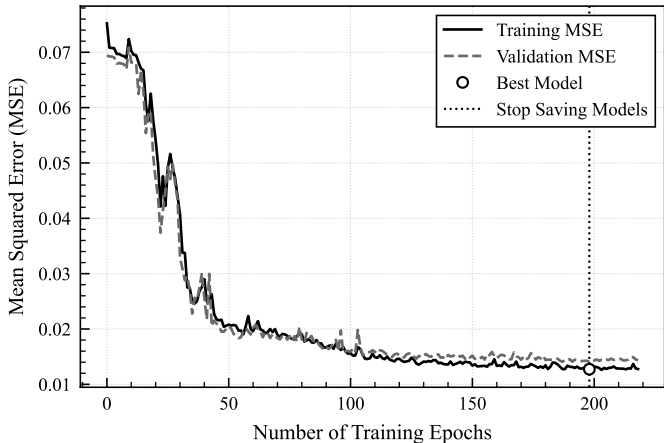
Learning Curve of TCSA-LSTM Model for SolarPlant-3 (Gyeongju)
